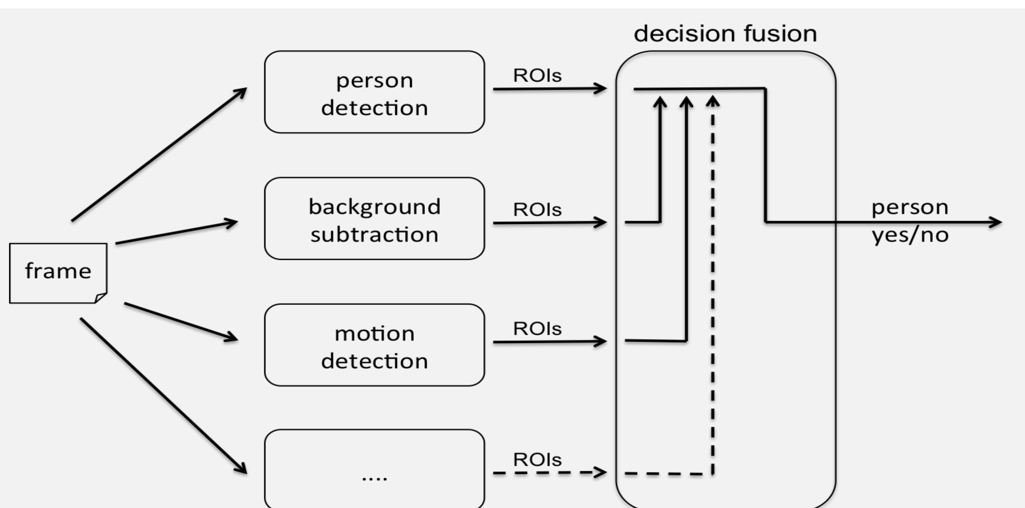
Fig. 2: Overview of the fusion process. The results of different modules are combined. Dependent on a computed score the process decides if a ROI can be discarded.
