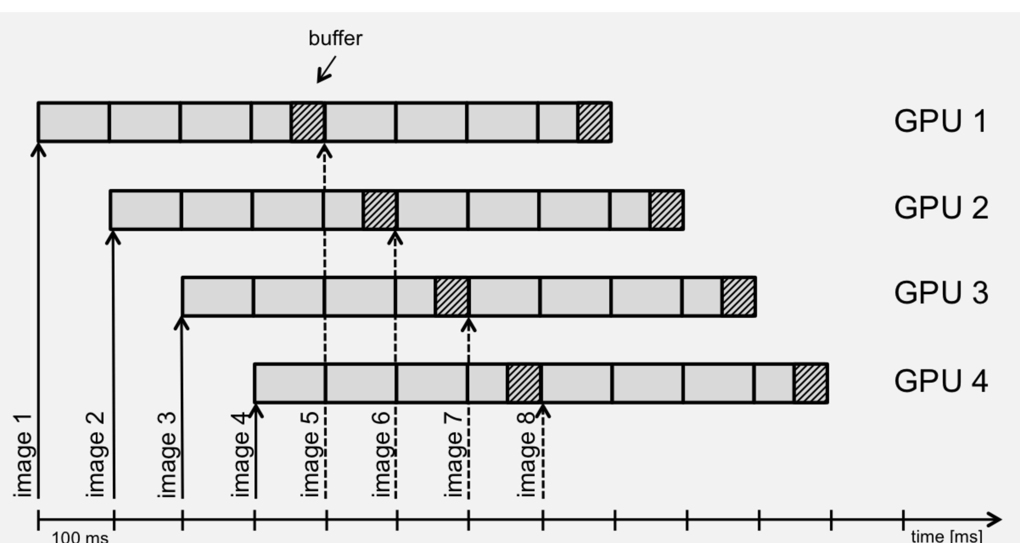
Fig. 4: Multi-Threading-Approach of a GPU-based person detection method. Each time an image is available, it is send to a free GPU which is then blocked until the processing has finished.
